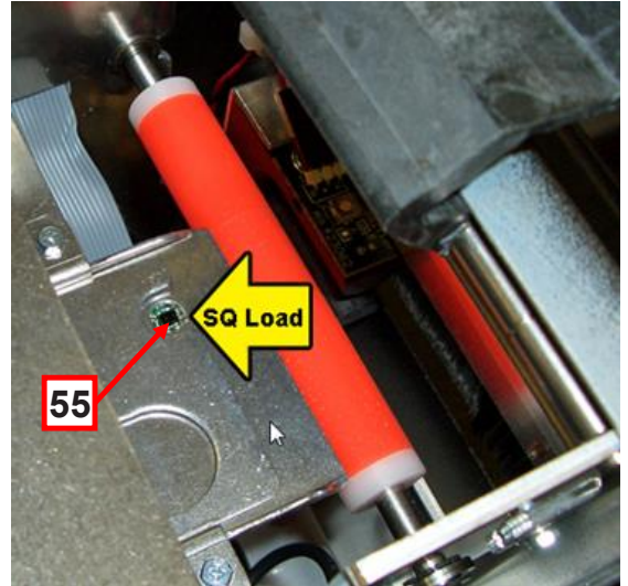
Above photo is of a Lemur-M built after February-2015 that has a SQ load opto. S/N 320833 & higher
