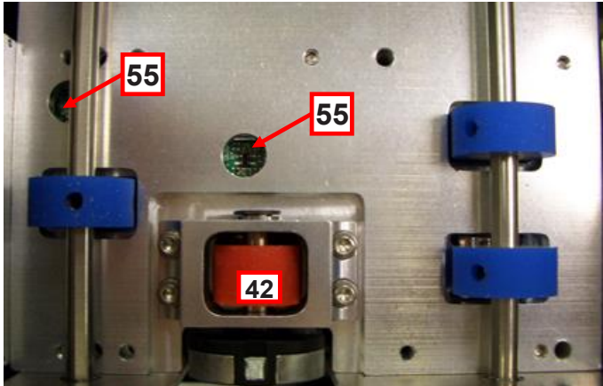
Above photo is of a Lemur-M or Lemur-MK with bottom encoding magnetic module. Printers S/N 356291 & higher.
