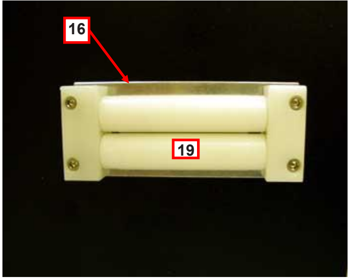
Ticket entrance of a Lemur-M with magnetic encoding
